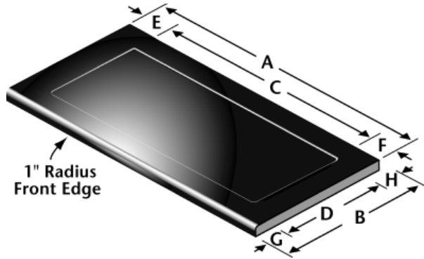
Contoura Fume Hood Base Dimensions
